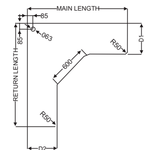
ANGULAR PROFILE
