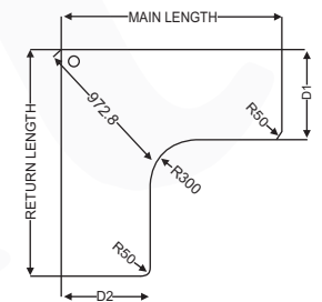
REGULAR PROFILE
