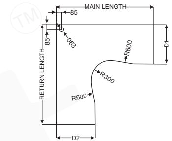
D-CURVE PROFILE
