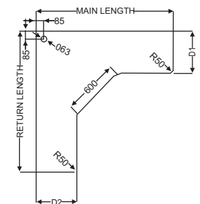
ANGULAR PROFILE
